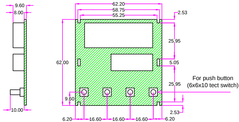
COMPONENTS P.C.B - 3 62x62.2
